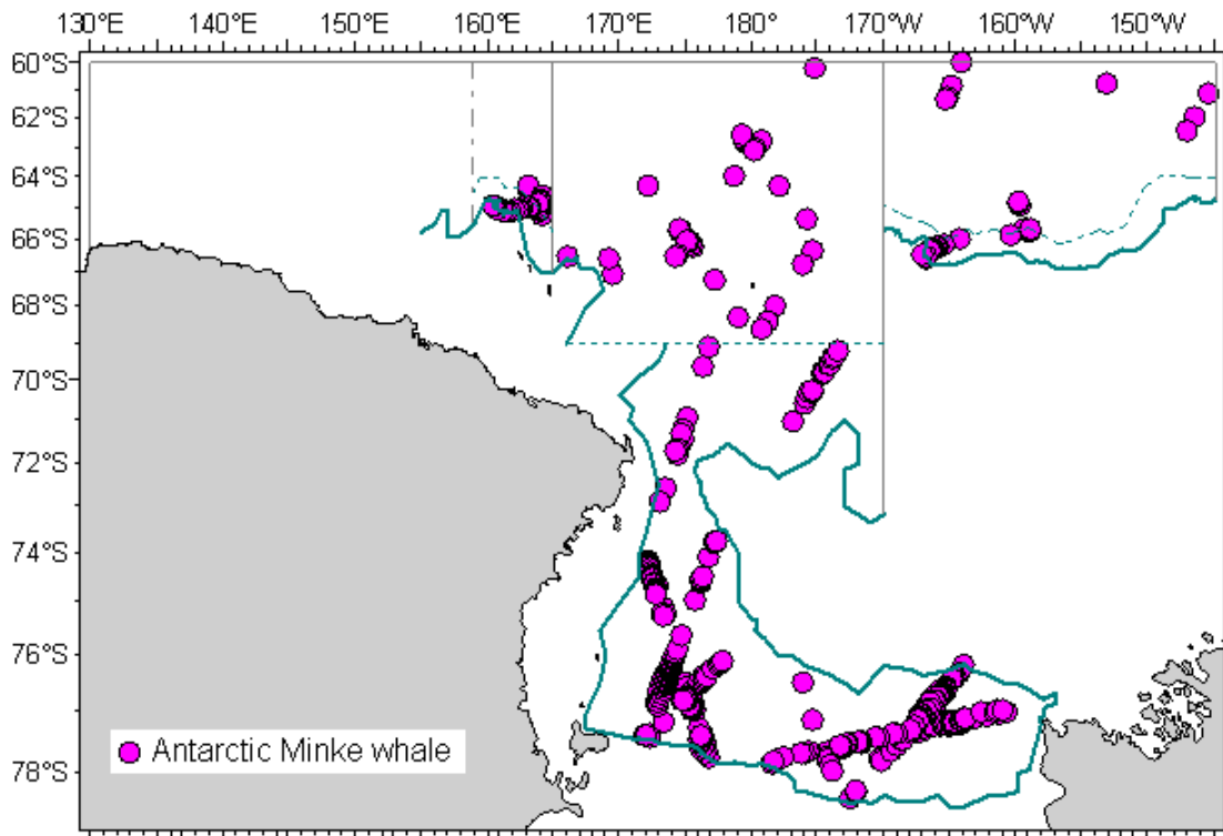
Figure 6. Distribution of primary sightings of Antarctic minke whales sighted by SVs in 2006/007 JARPAII.
