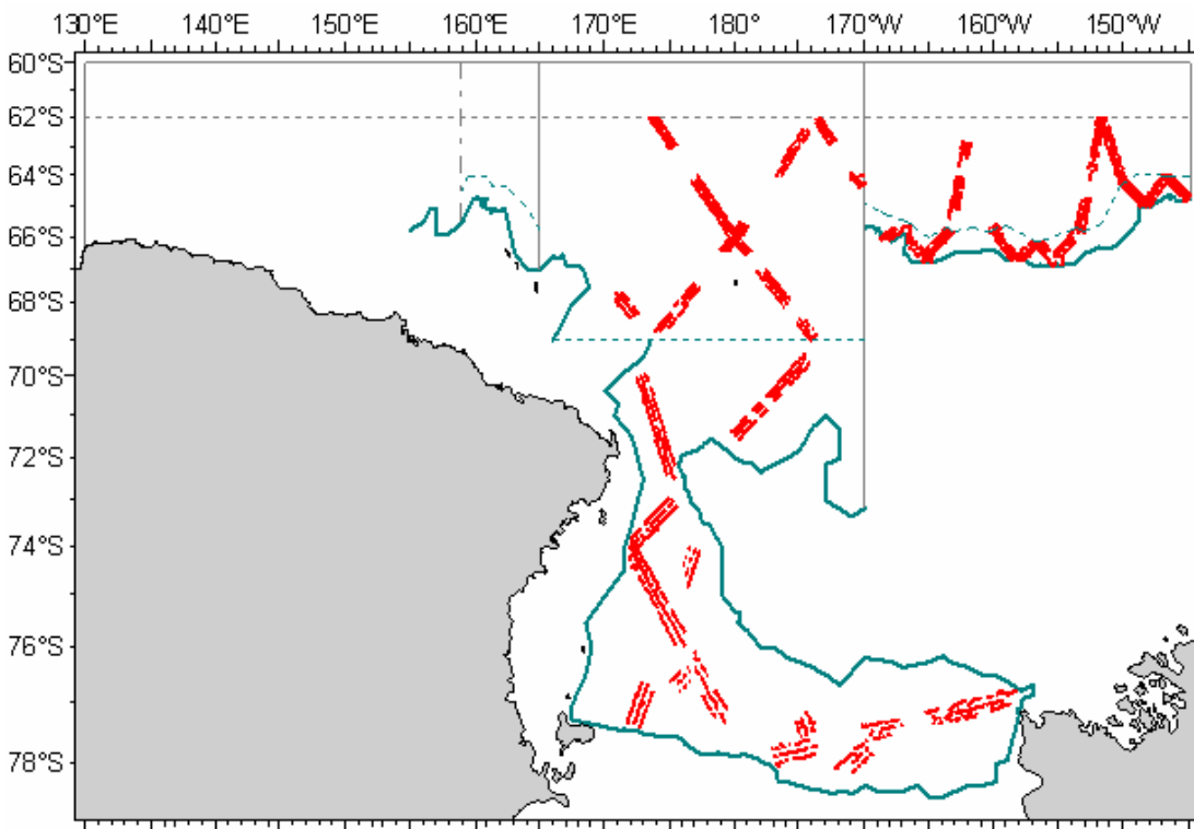
Figure 5. Survey track line of SSVs in 2006/2007 JARPAII.
