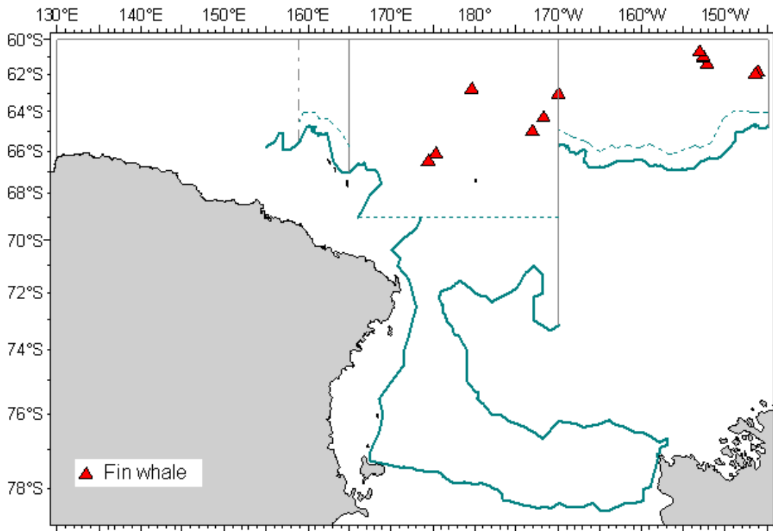
Figure 10. Distribution of primary sightings of fin whales sighted by SVs in 2006/2007 JARPAII.
