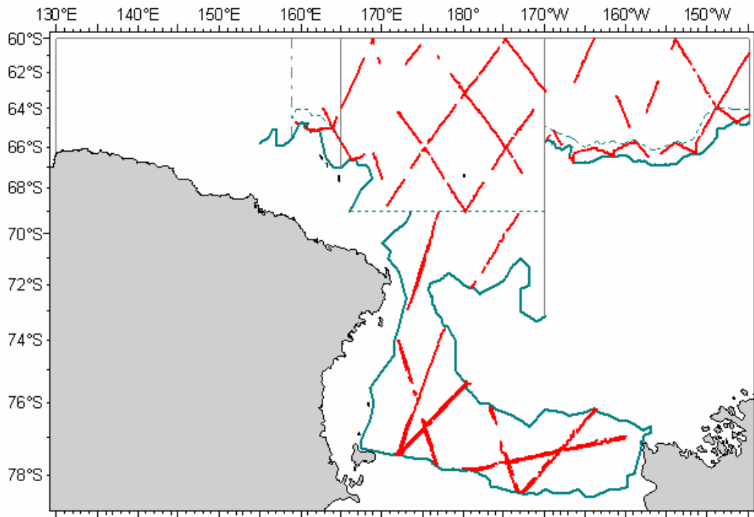
Figure 4. Survey track line Searching effort of SVs in 2006/2007 JARPAII.
