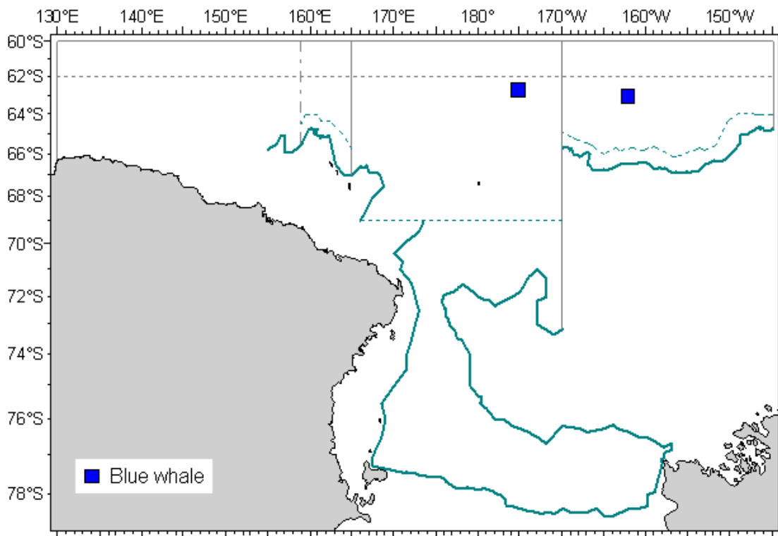
Figure 13. Distribution of primary sightings of blue whales sighted by SSVs in 2006/2007 JARPAII.
