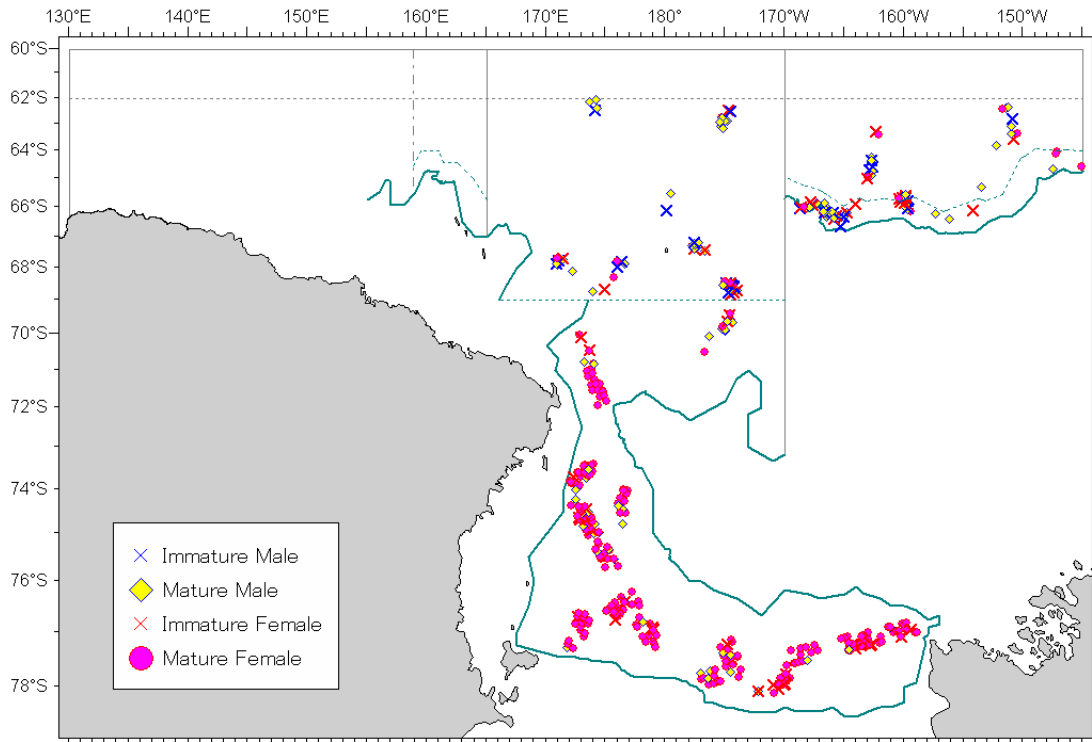
Figure 14. Sighted position of sampled Antarctic minke whales by sex and reproductive status in 2006/2007 JARPAII.
