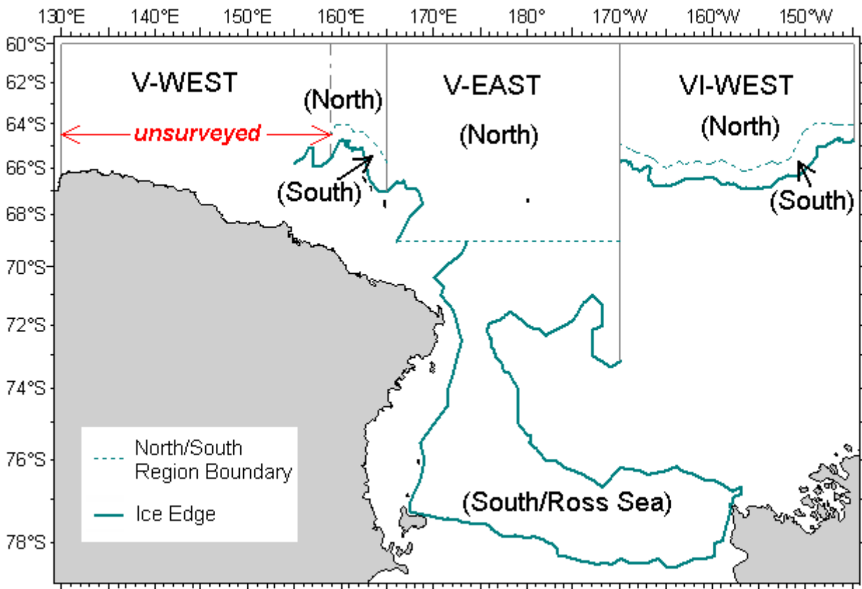
Figure 1. Geographic location of research area of the 2006/2007 JARPAII survey. Ice edge lines are estimated by observation from research vessels and the information from Near real time DMSP SSM / I daily polar gridded sea ice concentration data set available from the National Snow and Ice Data Center (NSIDC, Cavalieri et al. 1999).
