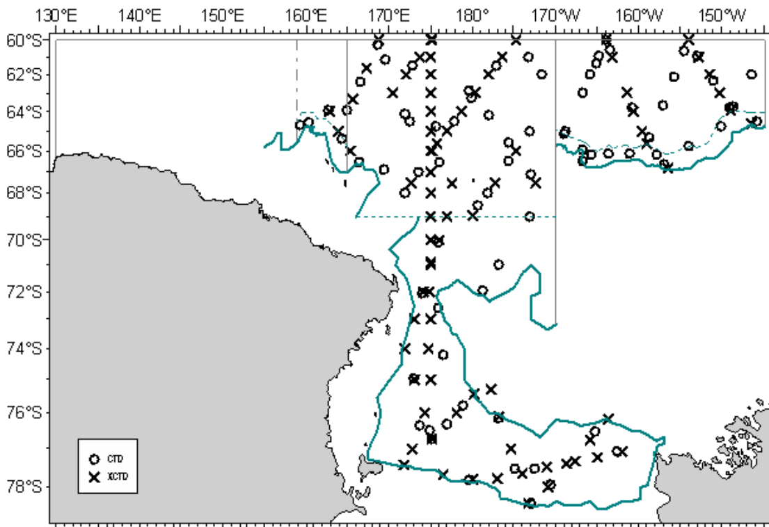
Figure 15. The CTD and XCTD observation stations in the research area in 2006/2007 JARPAII (circle: CTD stations, cross: XCTD stations).
